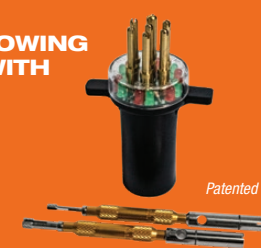
#7865L - 7-WAY ROUND PIN TRACTOR TRAILER CIRCUIT CHASER®
